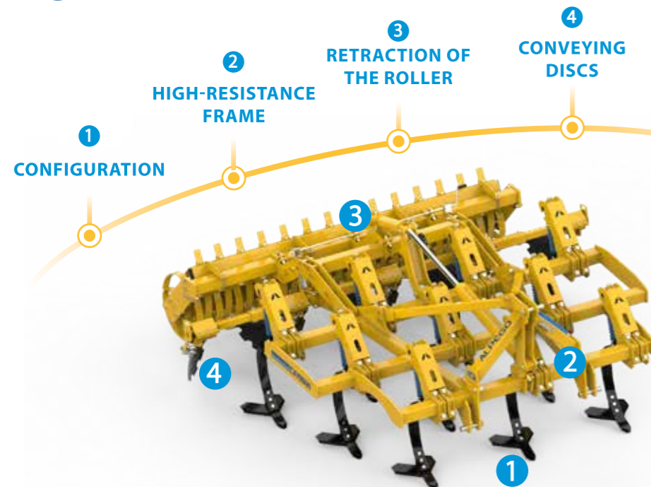
CA-300 TOP-MECC CA-350 TOP-MECC CA-300 TOP-SPRING CA-350 TOP-SPRING Working width (mm) 3000 3500 3000 3500 Transport width with rear roller (mm) 2980 3490 2980 3490 Tractor power (HP) 110-200 135-200 120-240 140-240 Working depth (mm) 300 300 300 300 Shanks (mm) 10 12 10 12 Distance between shanks (mm) 300 300 300 300 Weight with Cage roller (Kg) 1455 1665 1910 2155 Weight with Ring roller (Kg) 1710 1980 2160 2470 Weight with Disc roller (Kg) 1790 2040 2240 2580 Weight with Flex roller (Kg) 1670 1960 2120 2450
